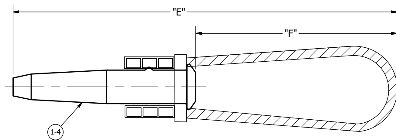
FIG 3 FLEX BAIL
