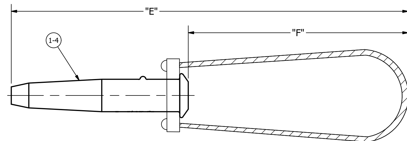
FIG 4 SEMI-FLEX BAIL
