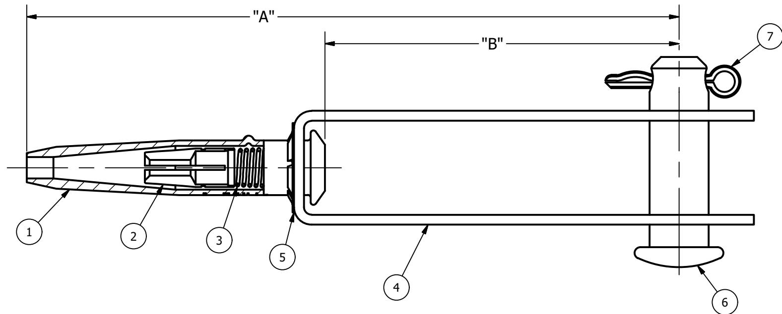
FIG 1 CLEVIS BAIL
